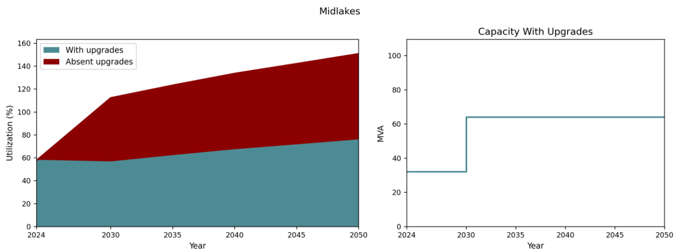
Figure 21. Midlakes Substation (2024 – 2050)
