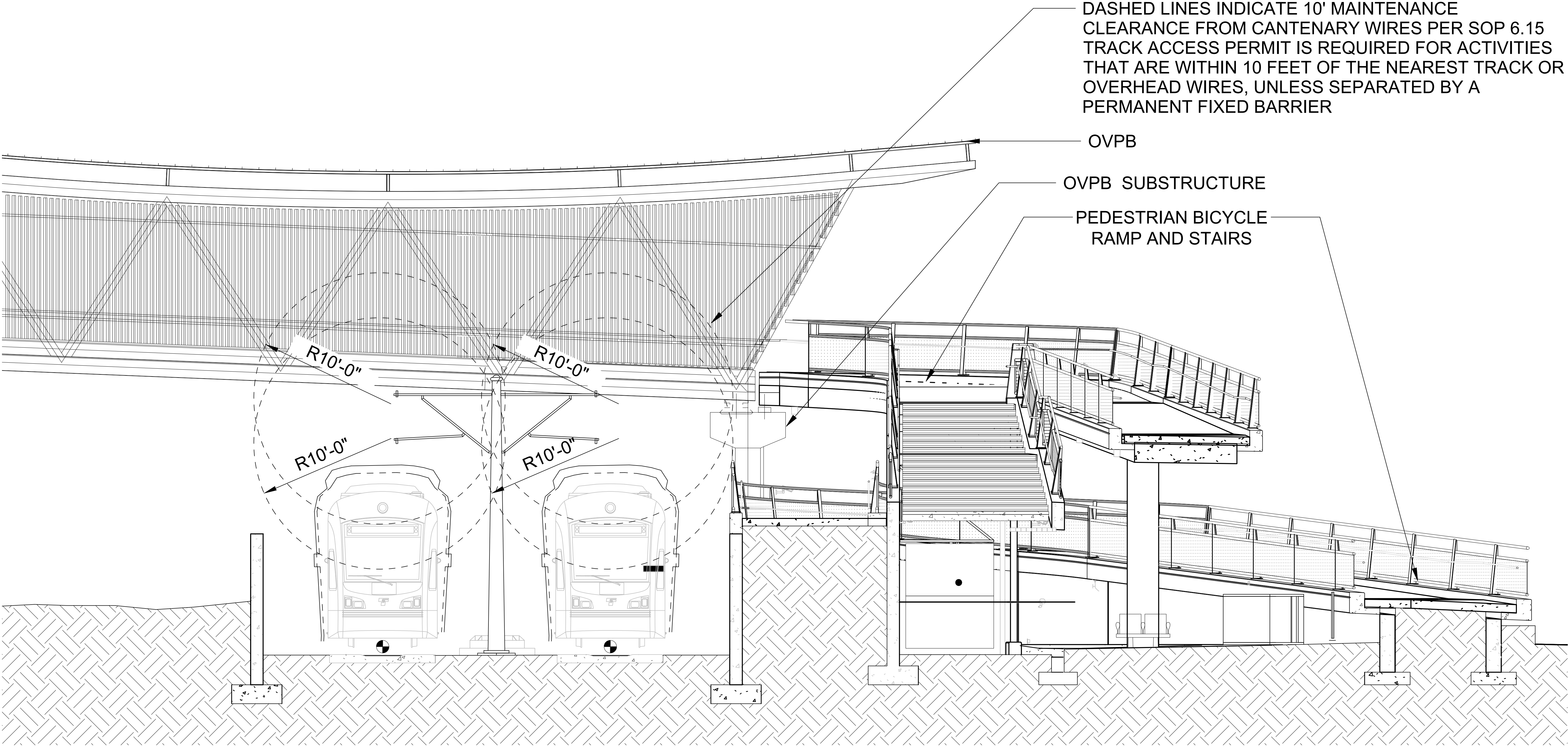
CROSS SECTION SCALE: 1/4" = 1'-0"
