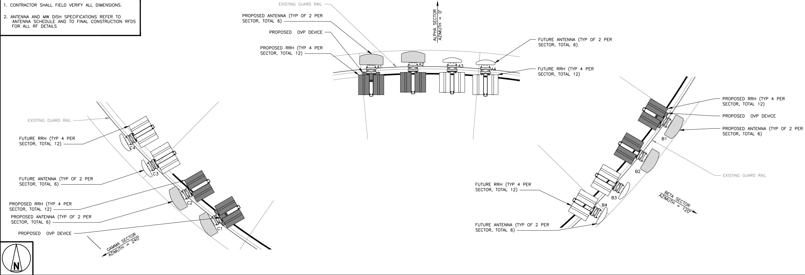
ANTENNA PLAN (TYPICAL PER SECTOR)
